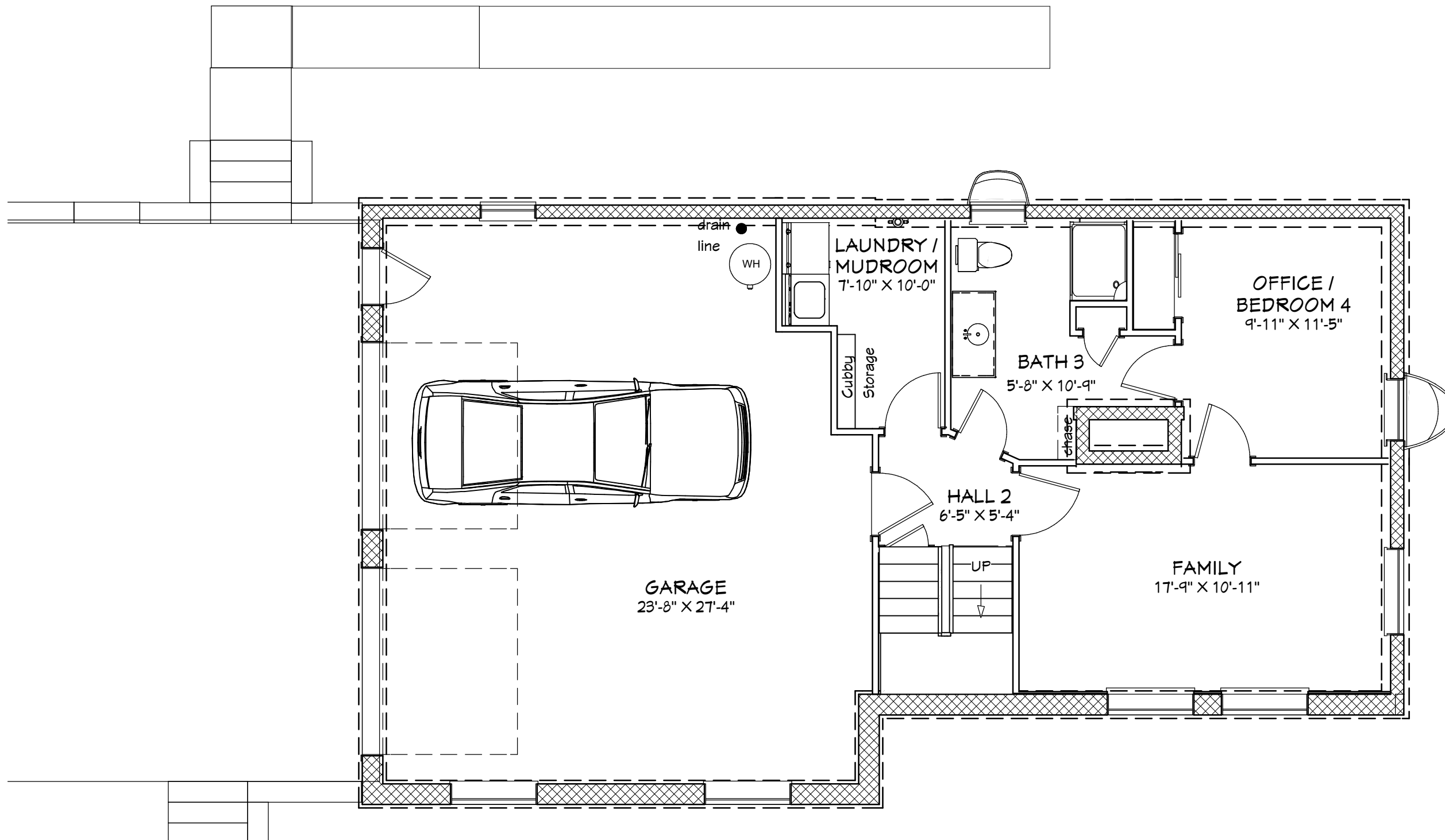
Lower Level Floor Plan
